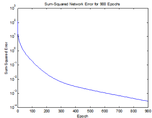
Figure 7b. SSE vs. Epochs for Fig. 7a.
