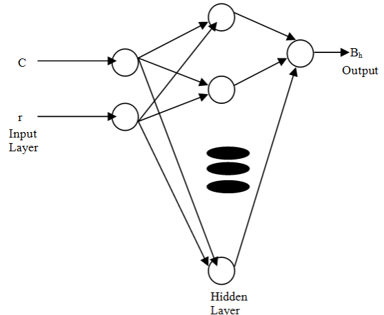
Figure 5b. ANN Model for calculating B_h taking C and r as inputs.
