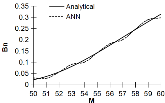
Figure 12a. B_n by varying M for FSM.
