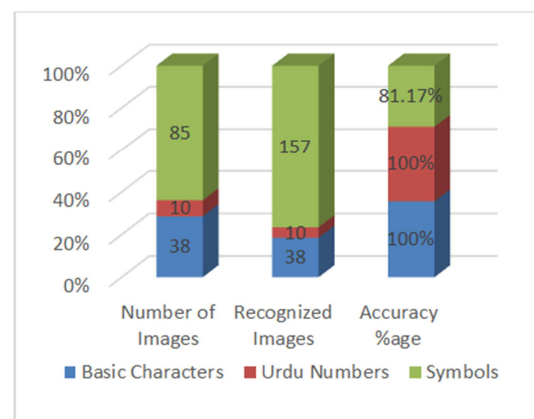
Figure 8. Basic characters.
