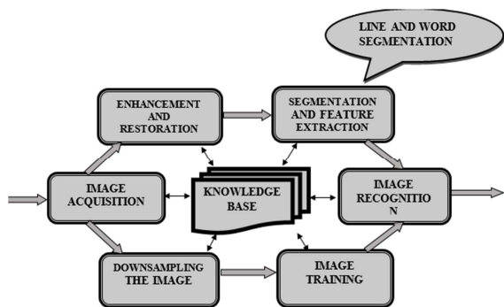
Figure 7. Knowledge Base.
