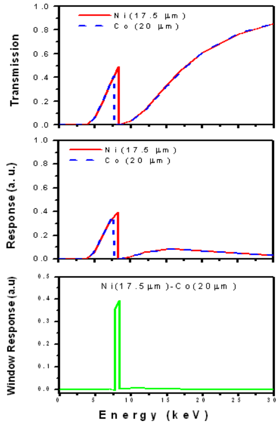
Figure 2. (a) Transmission curves of Ni ( 17.5 \mu\text{m} ) and Co ( 20 \mu\text{m} ). (b) Detector (PIN-diode) response along with corresponding filters. (c) Window response of Ross filters obtained by the subtraction of Co ( 20 \mu\text{m} ) from Ni ( 17.5 \mu\text{m} ) filter, the detector response is included.
