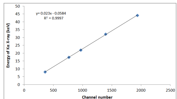
Figure (3-c). Energy of K_{\alpha} X-rays against channel numbers for Kr-detector
