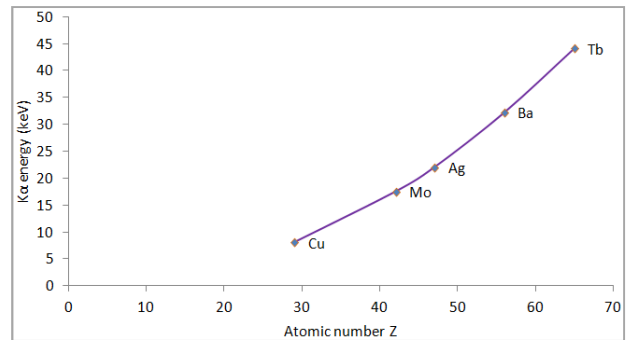
Figure (3-b). Average K_{\alpha} energy for the different elements against their atomic number.
