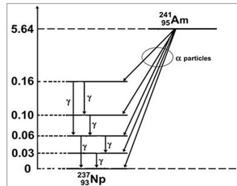
Figure (1-1). Schematic decay of ^{241}\text{Am} into ^{237}\text{Np} , taken from ( http://www.nap.edu/openbook.php?record_id=11976&page=2 ).
