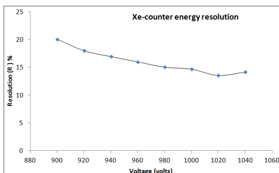
Figure (3-a). Energy resolution of the counters against applied voltage
