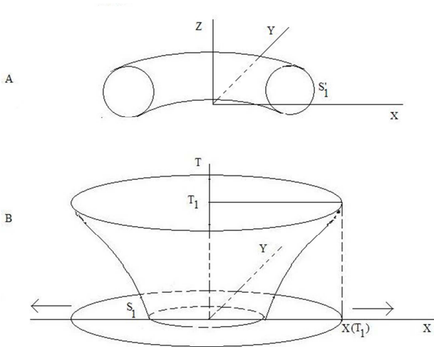
Figure 1. Geometrization of the free fermi-field (low-dimensional analogy).
