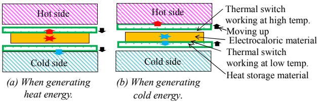
Figure 7. Model of electrocaloric refrigeration system with thermal switch by changing contact thermal conductance.
