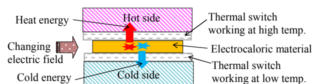
Figure 1. Model of electrocaloric refrigeration system.
