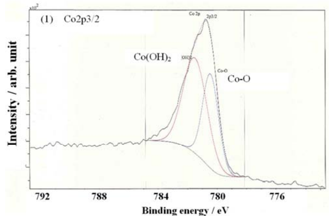
Figure 7. Co2p, O1s, Si2p, and N1s XPS spectra of thin cobalt film treated in 0.2% BTSPA-ethanol solution with hydrogen peroxide for 24 hours.
