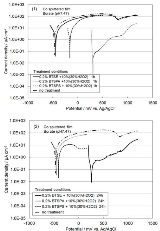
Figure 1. Polarization curves of sputtered cobalt films treated using several silane coupling-EtOH solutions with \text{H}_2\text{O}_2 for one hour (1) and 24 hours (2), as well as untreated cobalt films, measured in borate solution.
