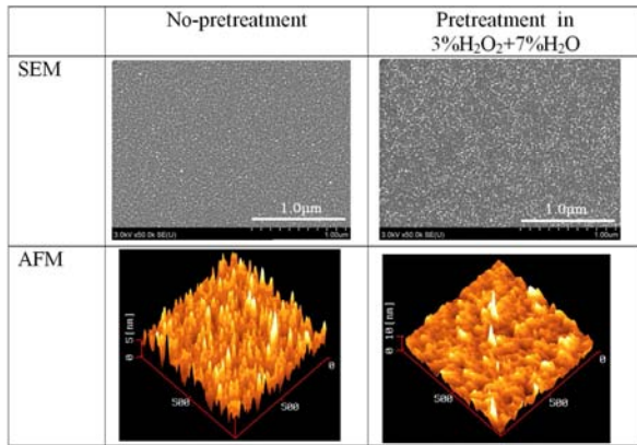
Figure 2. SEM and AFM images of thin cobalt film surfaces non-treated and treated in 3% H_2O_2 +7% H_2O +EtOH for one hour.
