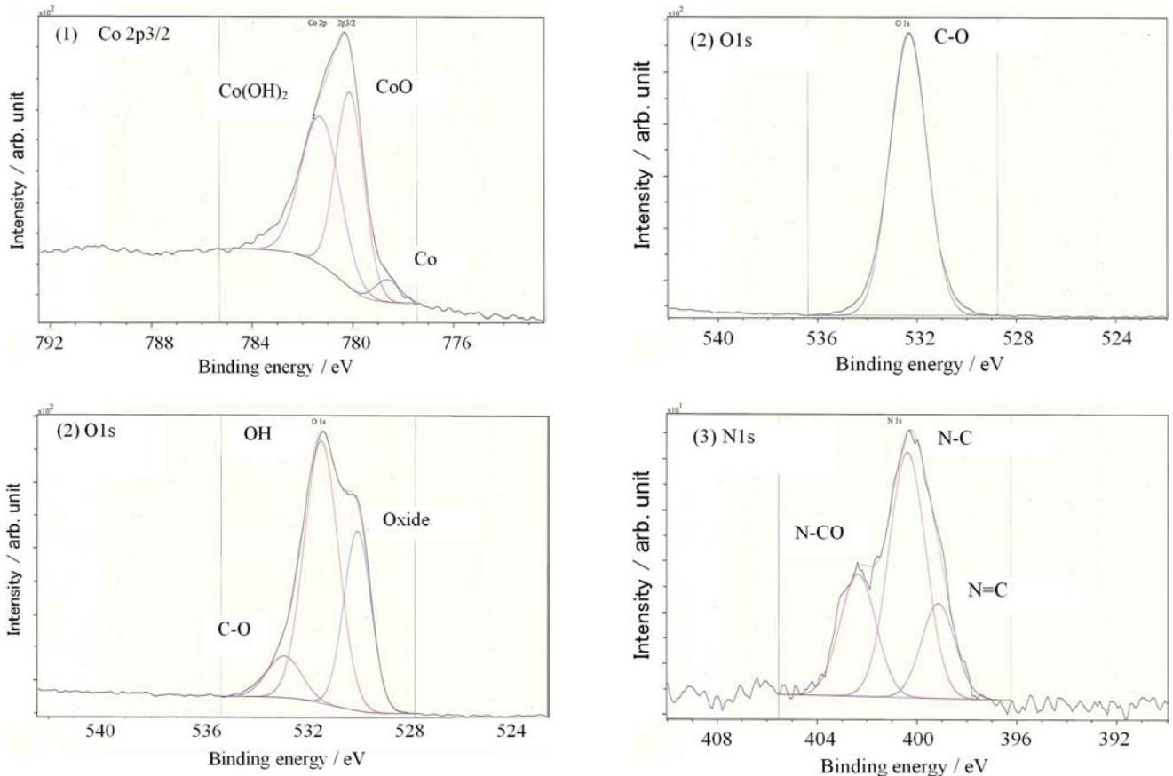
Figure 6. Co2p and O1s XPS spectra of thin cobalt film treated in BTSE-ethanol solution with hydrogen peroxide for 24 hours.
