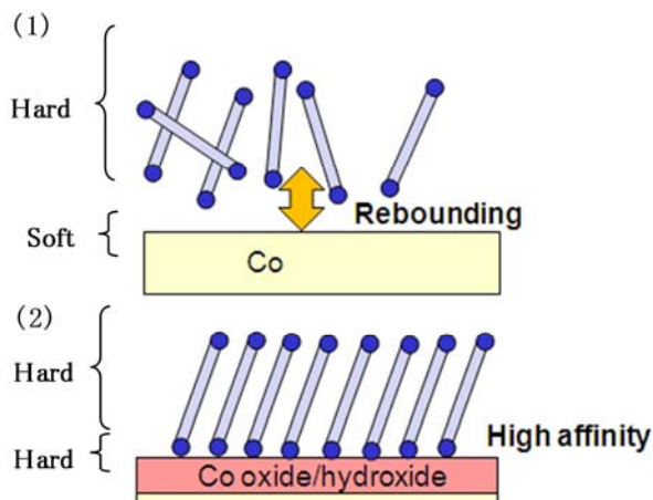
Figure 9. Adsorption model of BTSE on cobalt surface.
