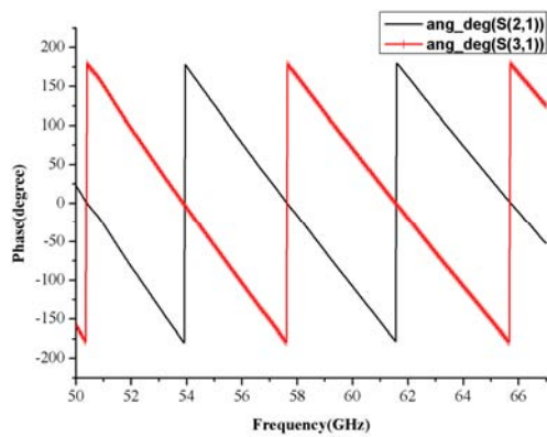
(b) Measured phase relation between two output ports of the waveguide power divider
