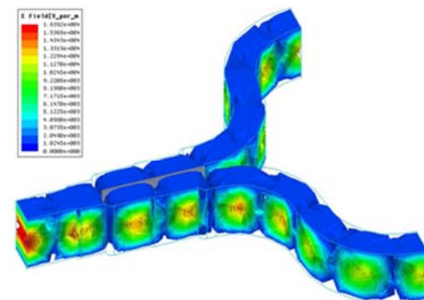
(b) Magnitude distribution of E field
