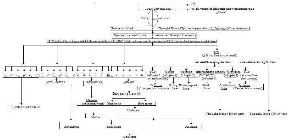
Scheme-I: Schematic representation showing the evolution of the universe from the void incorporating the postulated TCP (Thought carrying particle), TRP (Thought retaining particle), and thought force ( T_F ). Laws of absolute conservation of mass, charge (and color) are to be maintained in order to develop a general theory for the unification of physics which would be freely applicable to the more general situations involving the non-living system and living system having consciousness. Here TCP is the carrier of the thought force ( T_F ) that, in turn, is the origin of all the fields. TRP is the origin of all the matter particles. It is to be noted that these TCP and TRP function like wave-particle duality. Here thought force ( T_F ) is an expression of the "universal consciousness".
