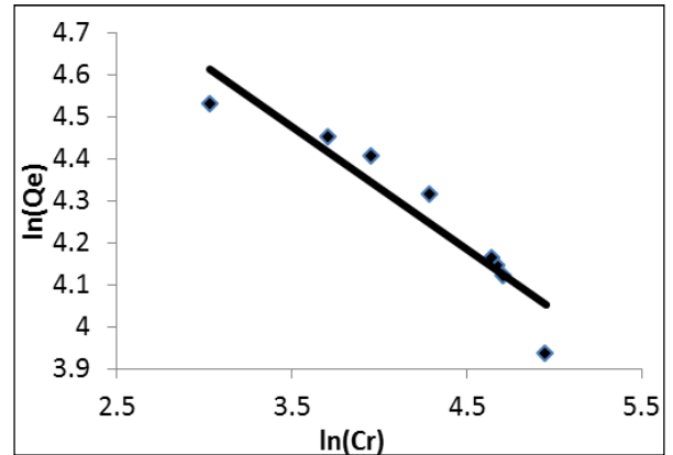
Figure 23. Linear Model of Freundlich.
