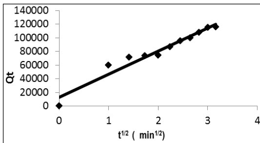
Figure 21. Intraparticle Diffusion Model.
