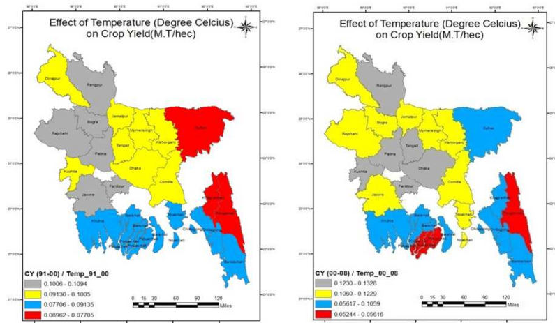
Figure 12: Effect of Temperature on Boro Yield (1991-00 and 2000-08)
