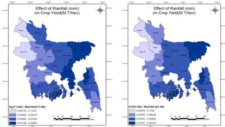
Figure 14: Effect of Rainfall on Boro Yield (1971-80 and 1981-90)
