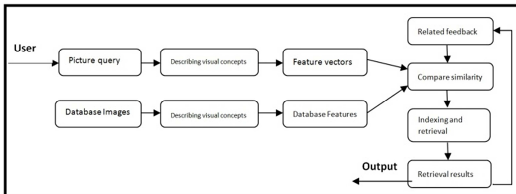
Figure 1. An example system architecture Content-Based Image Retrieval CBIR.
