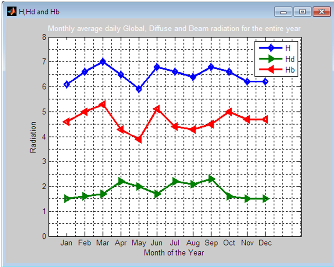
Figure 1. Monthly average daily Global, Diffuse and Beam radiations for the entire year.
