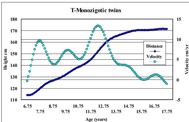
Figure 2. Height growth distance and velocity curve described by WIM in identical twins.
