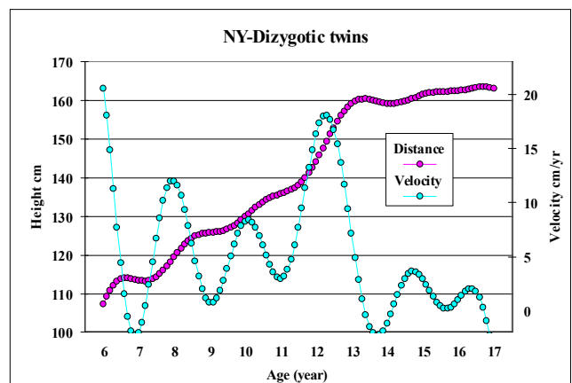
Figure 3. Height growth distance and velocity curve described by WIM in fraternal twins.
