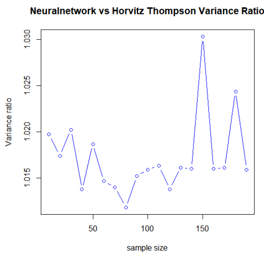
Figure 6. Variance ratio for neural network and HT estimators.
