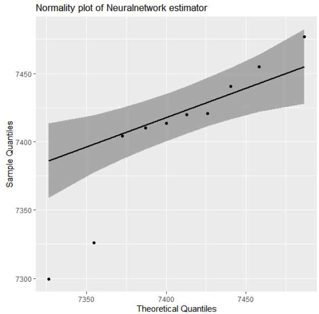
Figure 3. Normality plot for neural network estimator.
