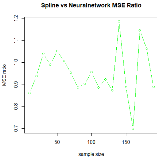
Figure 11. MSE ratio for spline and neural network estimators.
