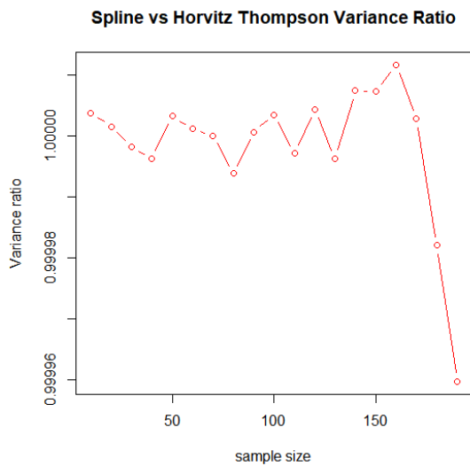
Figure 5. Variance ratio for spline and HT estimators.
