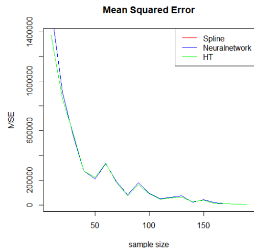
Figure 8. MSE for spline, HT and neuralnetwork estimators.
