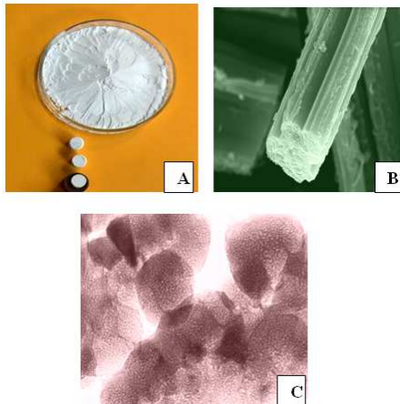
Fig. 1. Nanostructured 80% PSZ – 20% Al 2 O 3 powder: overview – A, microstructure of oxide monofiber – B (SEM x10000), nanostructure of powder particle – C (TEM x100000)
