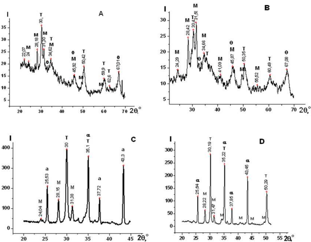
Fig. 2. X-ray grams of 20 % PSZ + 80 % Al 2 O 3 powder, synthesized at the 900 °C – A, blank after pulse pressing – B, ceramics annealed at the 1300 °C – C, ceramics annealed at the 1600 °C – D; M – monoclinic phase ZrO 2 , T – tetragonal phase ZrO 2 , θ – Al 2 O 3 , a – Al 2 O 3
