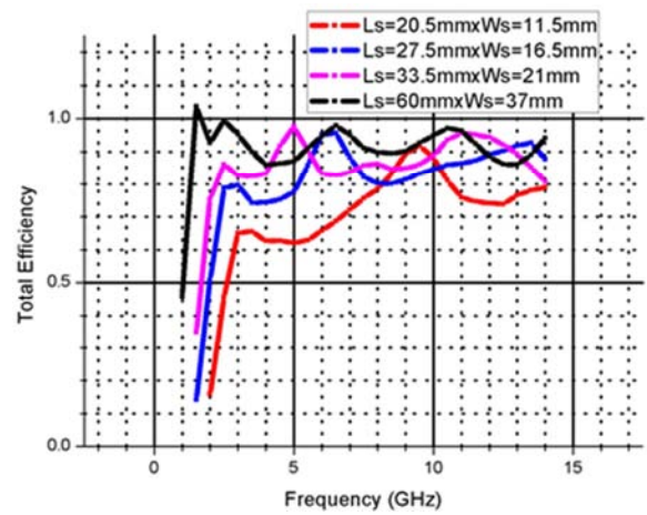
Figure 5. Simulated Results of Proposed Antenna with Reduced Size (case-2).
