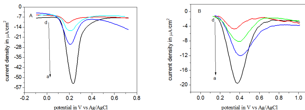
Figure 10. Differential pulse voltammograms obtained with GCE (A) and Pt (B) electrodes for different ascorbic acid concentrations, expressed as mM: (a)12(b) 10(c) 8 and (d) 6; experimental conditions: pulse amplitude 50 mV; pulse period 125 ms, potential scan rate 50mV/s.
