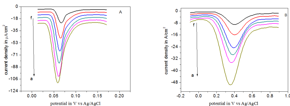
Figure 12. Influence of pulse amplitude of DPV on ascorbic acid determination, using GCE (A) and Pt (B) electrodes; (a) 25 mV(b) 50 mV(c) 75 mV(d) 100 mV(e) 125 mV and (f) 150 mV; experimental conditions: pulse period 125ms, potential scan rate 50 mV/s.
