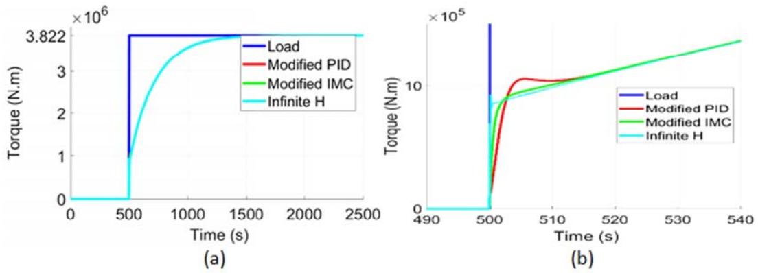
Figure 17. The load moments and torques on the alternator shaft, (a) normal, (b) zoom.
