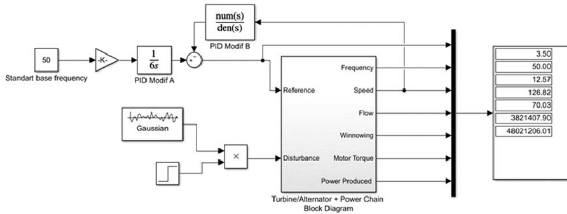
Figure 10. Model of the power plant in the presence of the modified.
