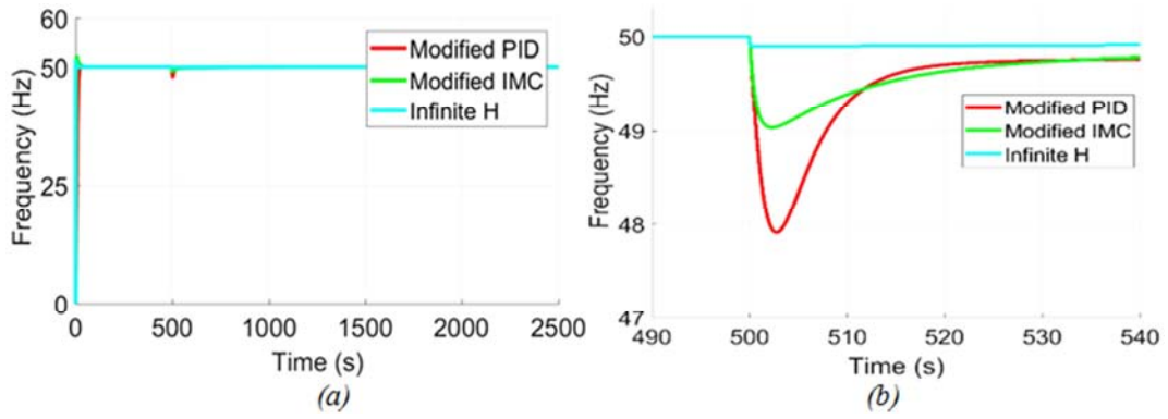
Figure 15. Frequency output of the alternator with controller; (a) normal, (b) zoom.
