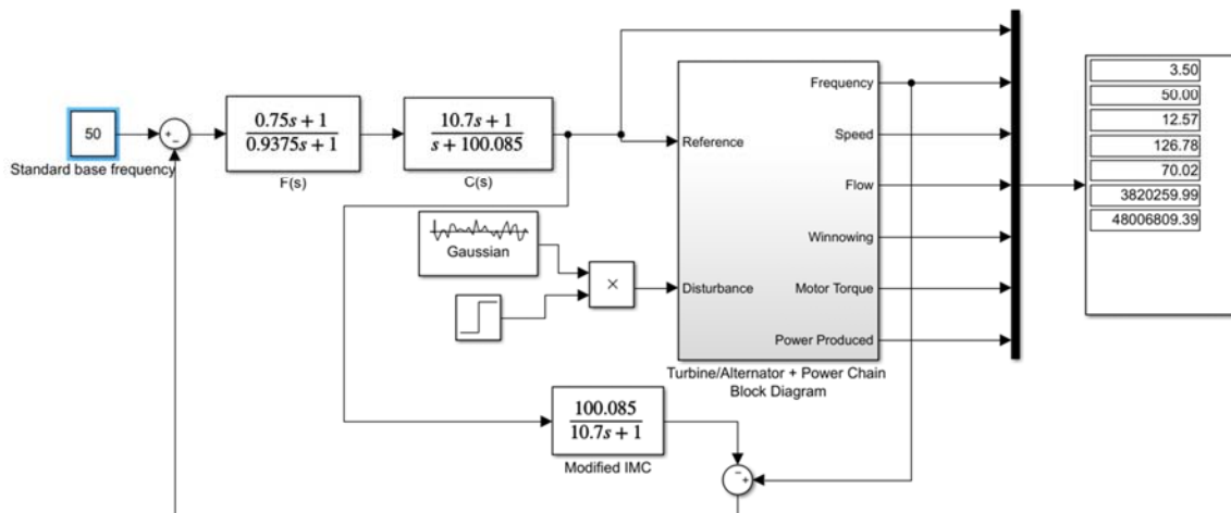
Figure 11. Model of the power plant in the presence of the Modified IMC controller.
