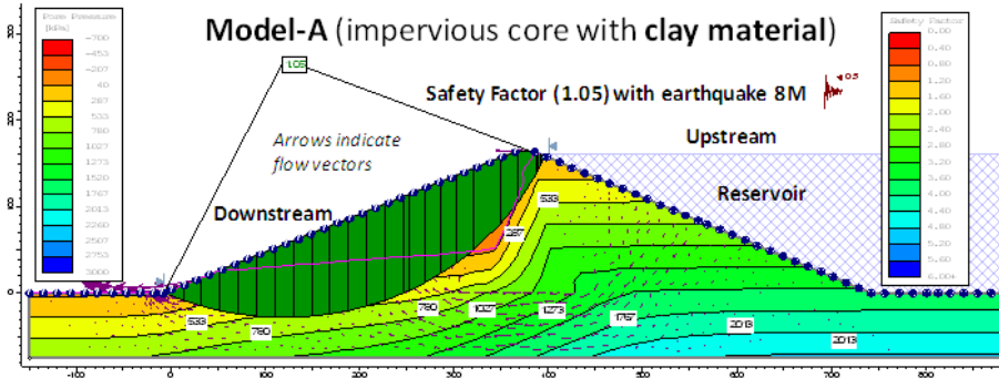
Figure 11a. Safety factor of the Tipaimukh Dam with earthquake magnitude 8.0 (model A)
