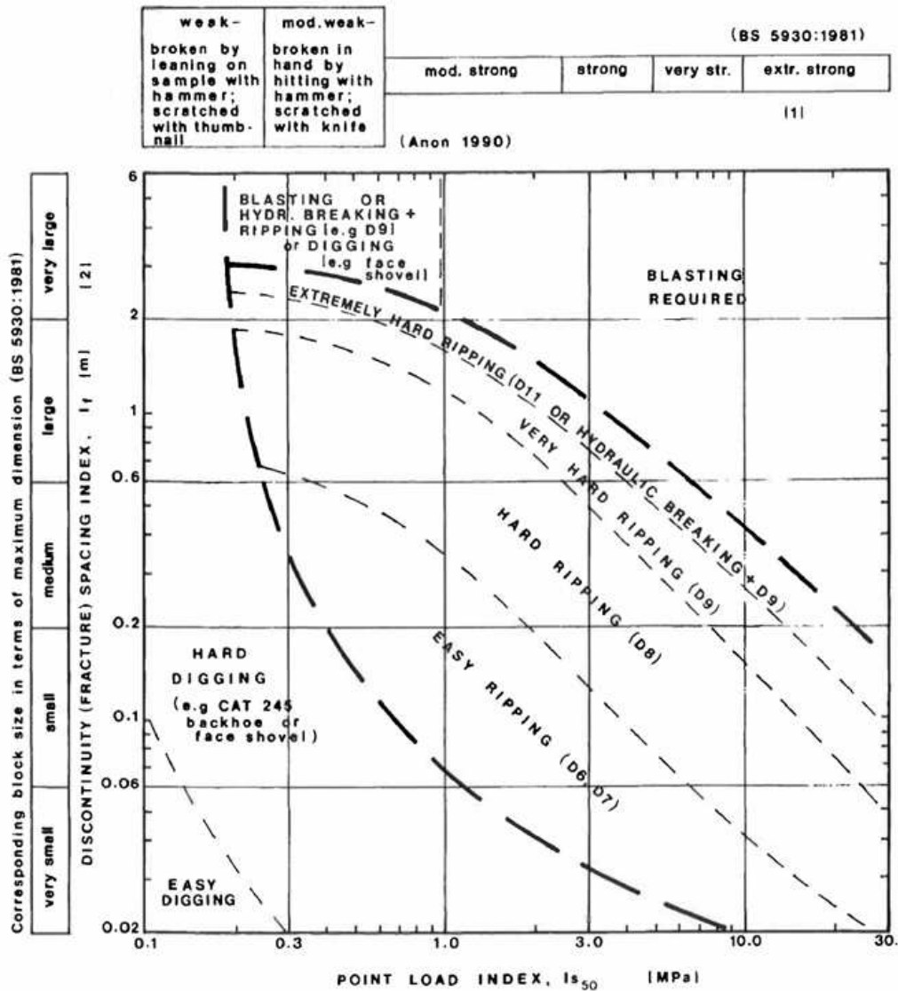
Figure 3. Excavatability Assessment Chart (Pettifer and Fookes, 1994)
