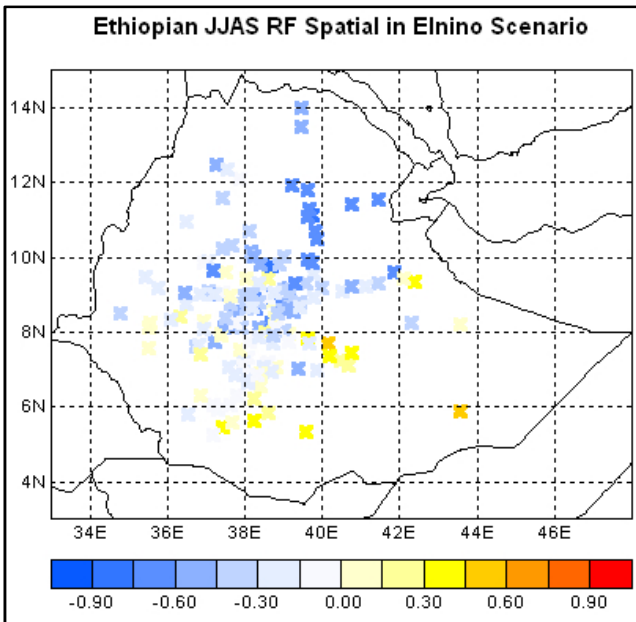
Figure 8. spatial loading pattern relating Ethiopian JJAS rainfalls to tropical SST, for (top) El Niño and (bottom) La Niña.
