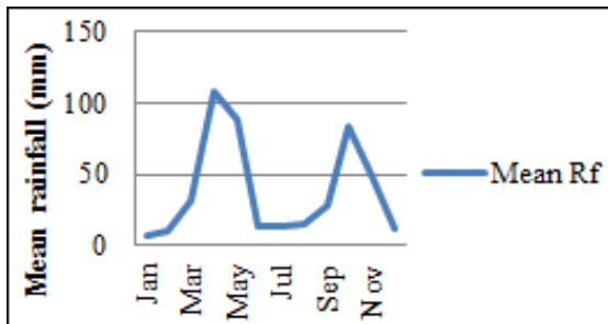
Figure 4. Ethiopian annual cycle of Rainfall (mm), 1970-2006: (top) northeast, east and central, and (bottom) south and southeast.
