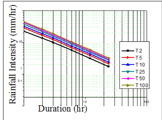
c) IDF for 2050s scenario hurso
