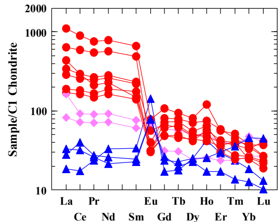
Figure 18. Chondrite normalized pattern for the studied Gabal Adara Adatalob granite.
