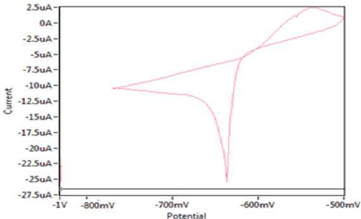
Figure 12. Cyclic voltammogram of 10mM Pb(II) in normal saline as an electrolyte in present of 10mM urea by GCE at scan rate 100mVsec -1 versus Ag/AgCl as reference electrode.
