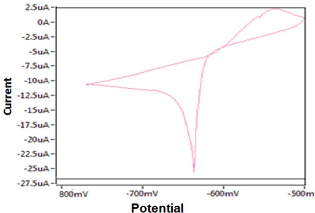
Figure 9. Cyclic voltammogram of 10mM Pb(II) in normal saline as an electrolyte in present of 10mM uric acid by GCE at scan rate 100\text{mV}\text{sec}^{-1} versus Ag/AgCl as reference electrode.
