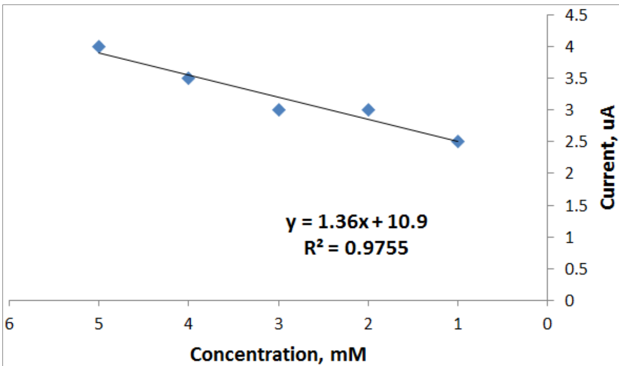
Figure 11. Plotting of cathodic current peak of Pb(II) in different concentrations of uric acid using normal saline as supporting electrolyte.
