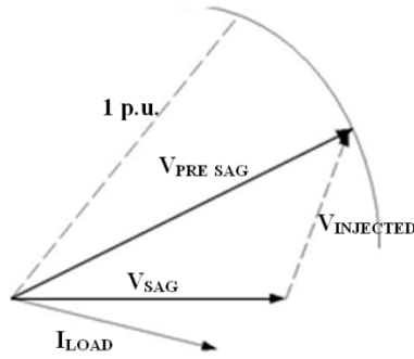
Figure 2. Pre-Sag Compensation Method.
