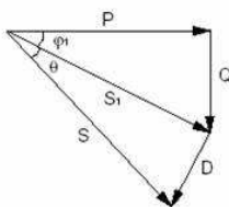
Figure 4. Reactive Power Compensation.
