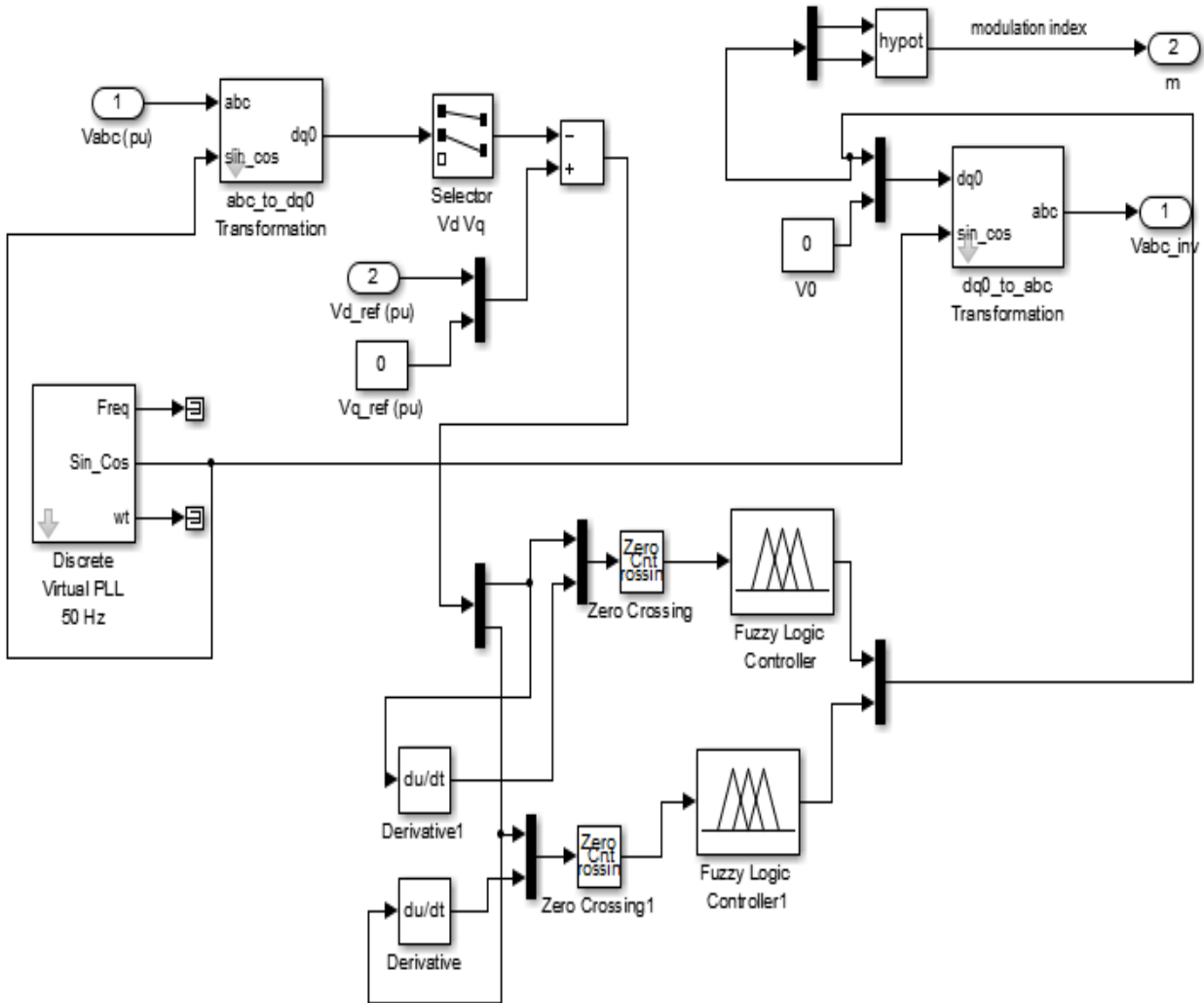
Figure 10. Control Strategy of Fuzzy Controller.
