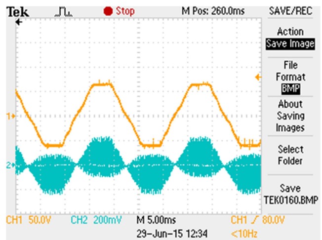
Figure 8. CH1- input voltage, CH2 – inductor current – 2A/div.
