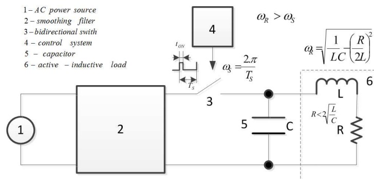
Figure 1. Block diagram of the new AC-AC quasi-resonant converter.
