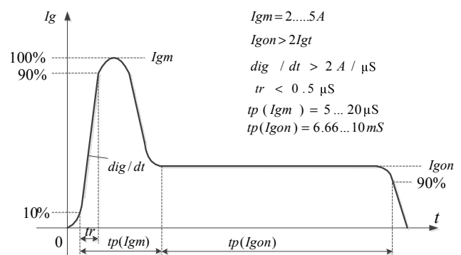
Figure 1. Requirements to the control pulse waveform.
