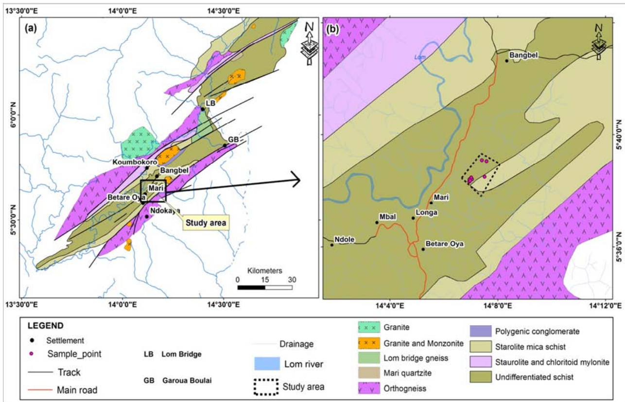
Figure 1. Regional Geologic setting of study area.
