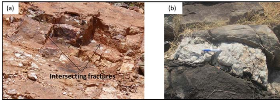
Figure 4. (a) Mineralized vein dissected by intersecting fractures (b) Non-Mineralized vein.
