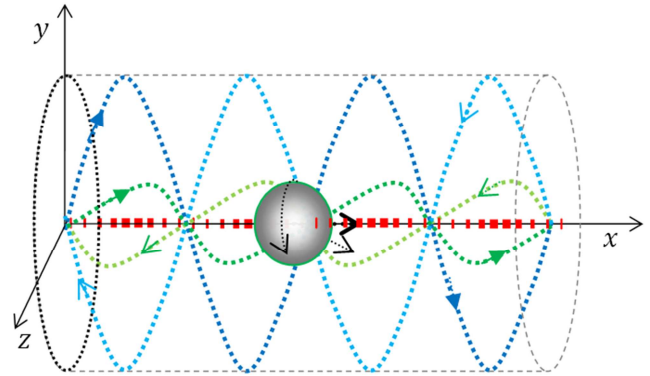
Figure 2. Three kinds of wave propagation along x -direction: the sphere represents the particle at a given position; its size is only illustrative and the associated arrows try to indicate the resulting vector between the spin momentum (horizontal) and the orbital one (transverse), foreseeable from the wave function microscopy. The short vertical lines represent the case of one longitudinal wave. The vertical or horizontal sinusoids delimit the cases of transverse waves. The arrows indicate the possible propagation senses in interference case.
