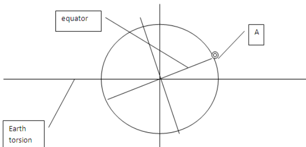
Fig 4. Inclination of the Earth's equator.
