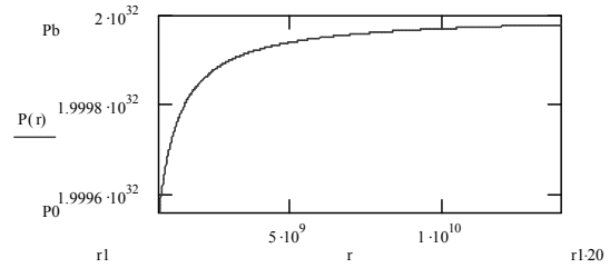
Fig 2. The radial distribution of the ether pressure for the Sun.
