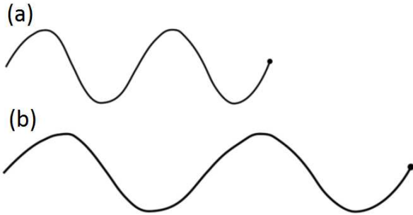
Figure 1. Light wavefront. Where (a) is the light wavefront without stretching, and (b) with stretching. We can see that in (b) the light wavefront is going faster than in (a).
