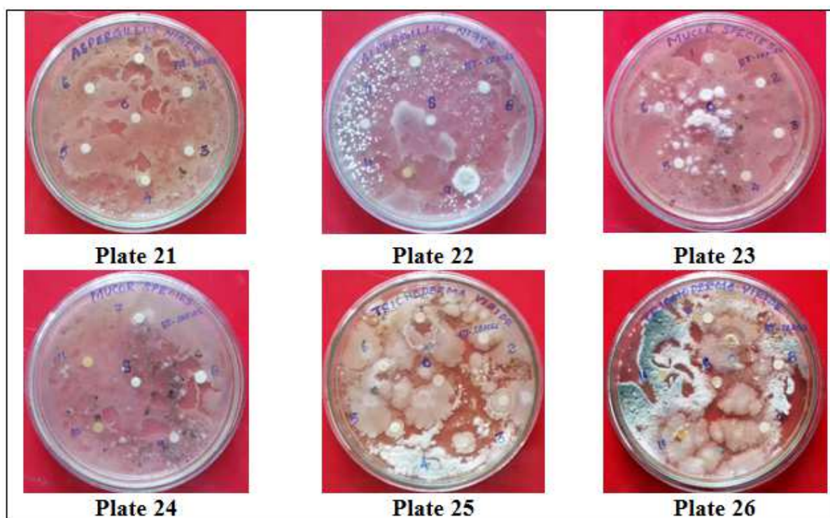
Figure 4. Antifungal sensitivities of substituted ( E )-3-(5-bromothiophen-2-yl)-1-phenylprop-2-en-1-one compounds.
