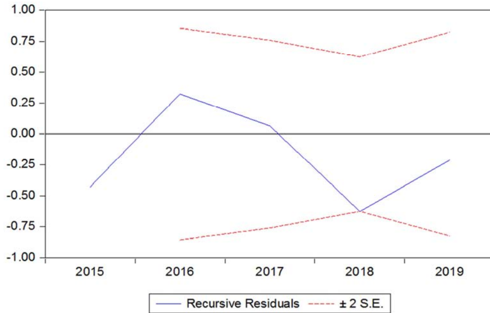
Figure 5. Recursive Residuals.
