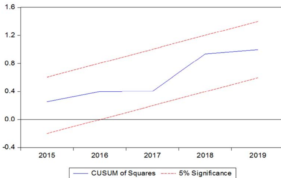
Figure 4. CUSUM of Squares of Residuals.
