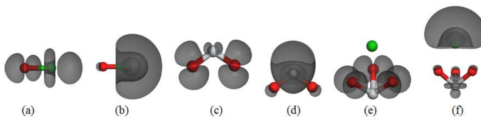
Fig. 8. The HOMO and LUMO orbitals of BaO, TiO 2 , and BaTiO 3 molecules (color online).
