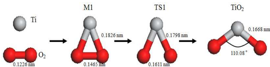
Fig. 1. The process of formation of molecular TiO 2 (color online).
