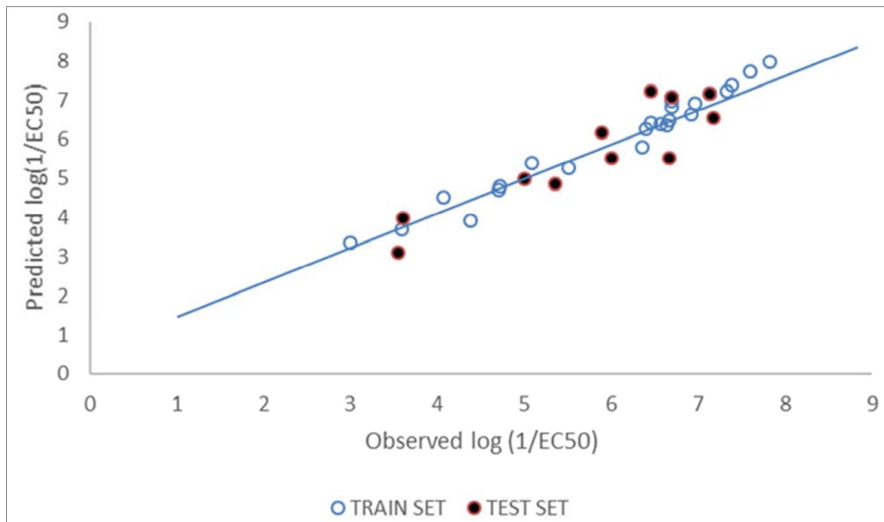
Figure 2. Plot of predicted (Training & Test sets) versus the observed log (1/EC50) values.
