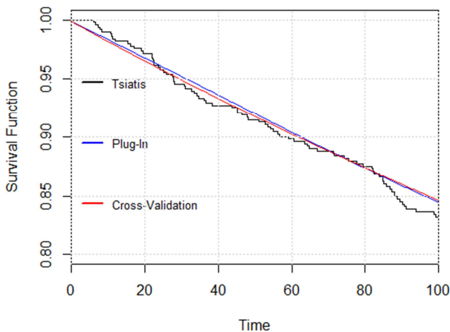
Figure 1. Tsiatis, Cross-Validation and Plug-In survivorship functions.
