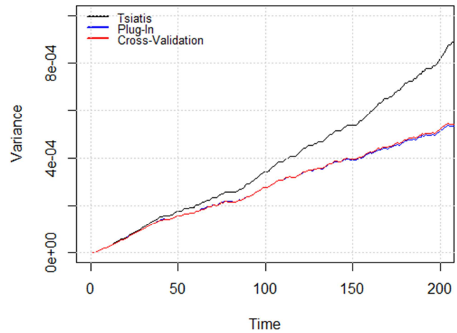
Figure 2. Point-wise asymptotic variance estimates for the survivorship function.
