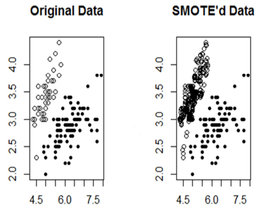
Figure 1. The plots of original data and "SMOTE'd" data.
