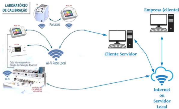
Figure 2. Calibration procedure 4.0. [8]
