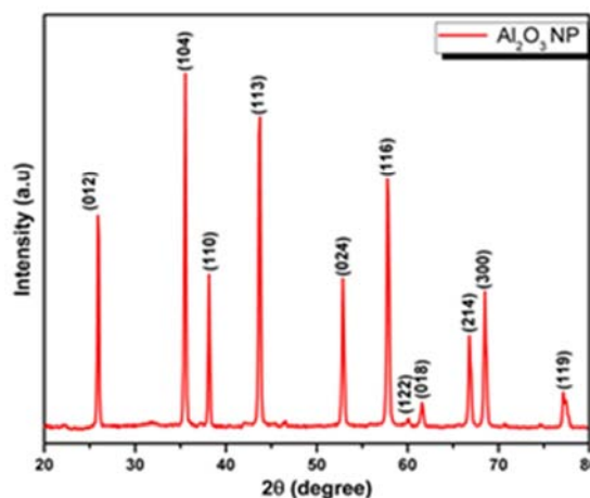
Figure 11. XRD of Al_2O_3 Nanoparticles.
