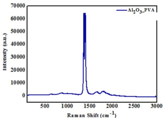
Figure 10. Raman Spectra of Al_2O_3 Nanoparticles.
