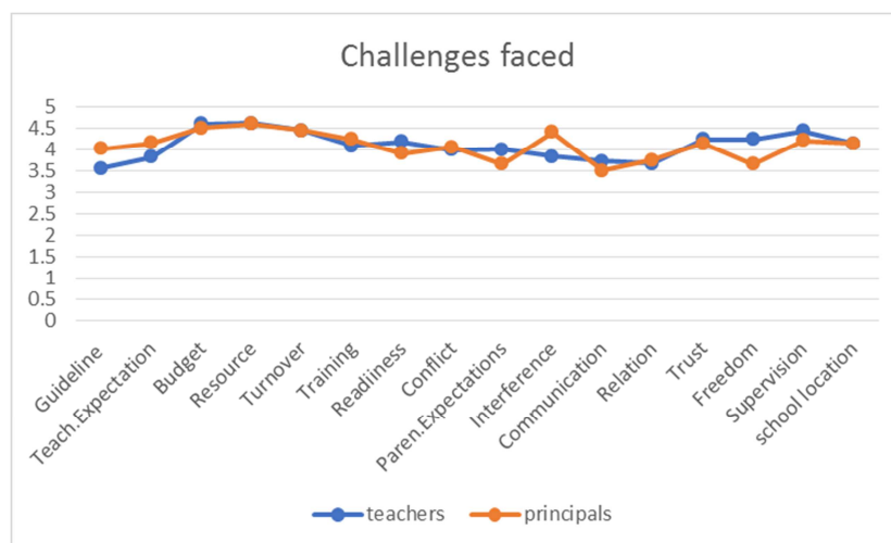
Figure 2. Challenges faced.
