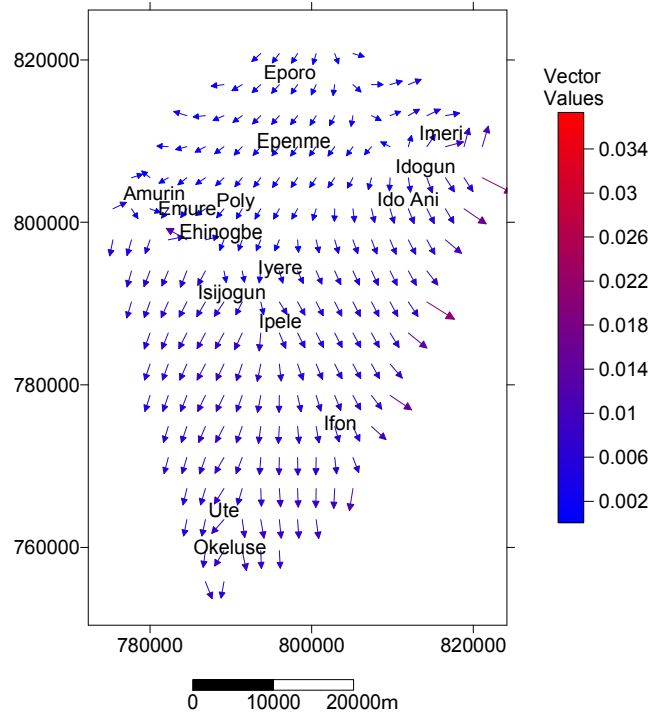
Figure 5. 1-Grid Vector Map showing potential Groundwater flow direction.
