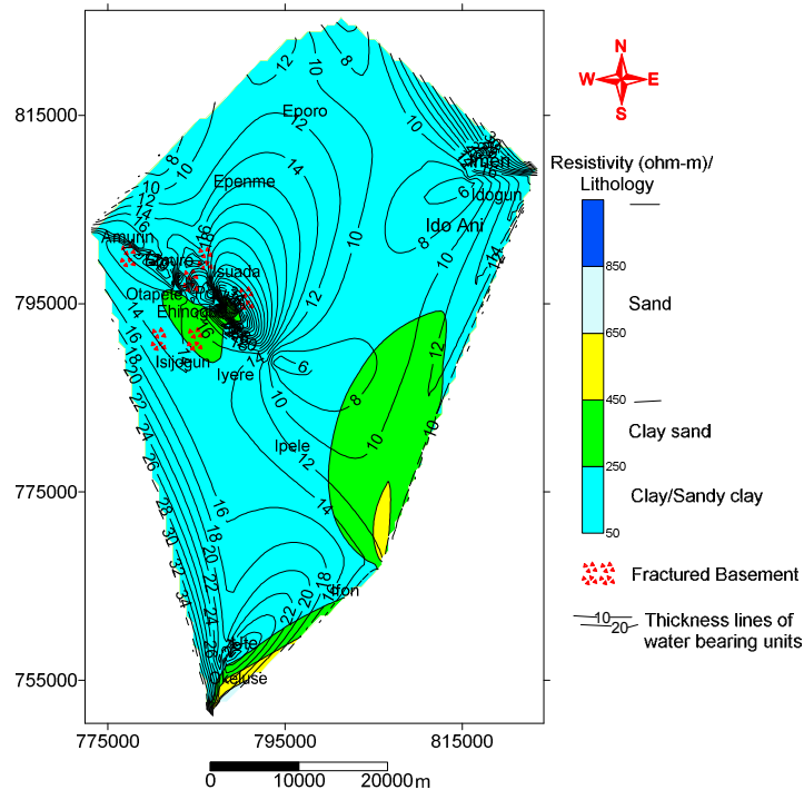
Figure 10. Map showing water bearing units and their corresponding thickness.
