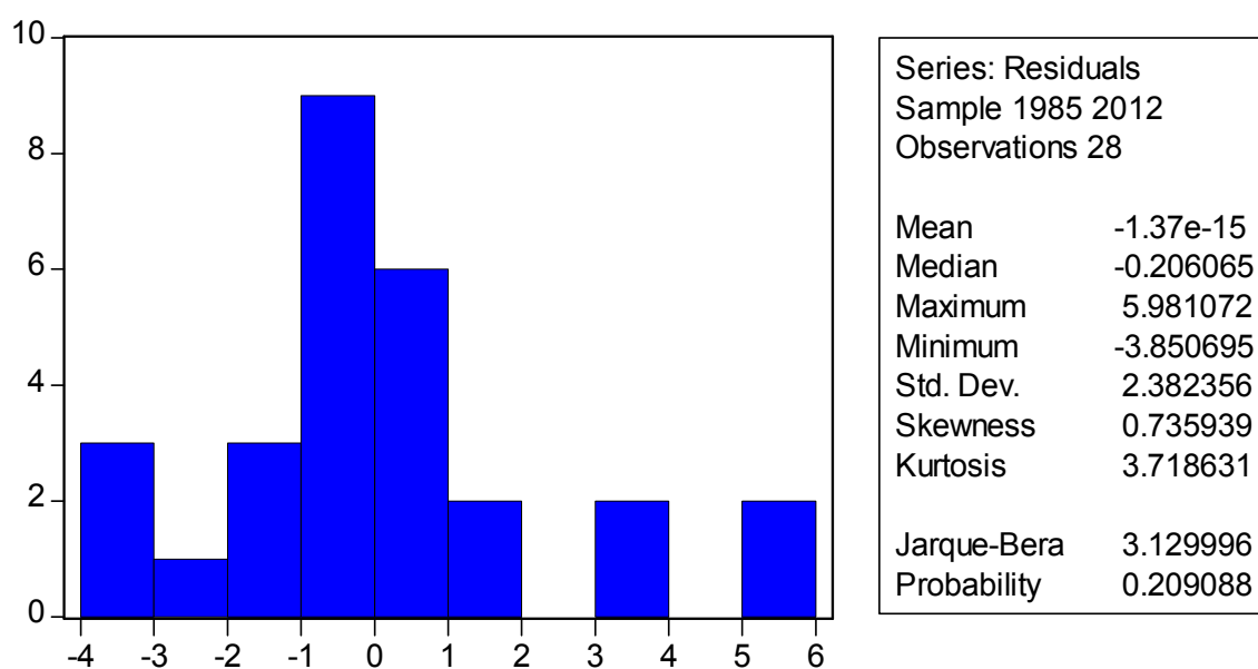
Figure A3. Normality Test for model 3.
