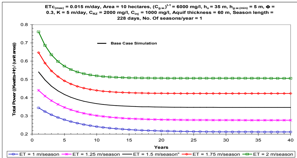
Figure 3. Total power required by the system for ranges of different actual crop evapotranspiration, ET_c , input values vs. simulation period.
