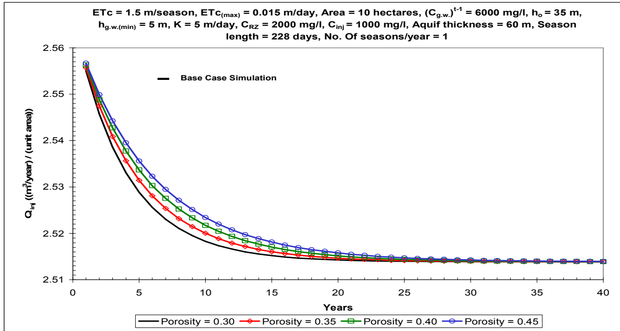
Figure 10. Amount of treated wastewater injected into the native groundwater for ranges of different porosity, \Phi , input values vs. simulation period.
