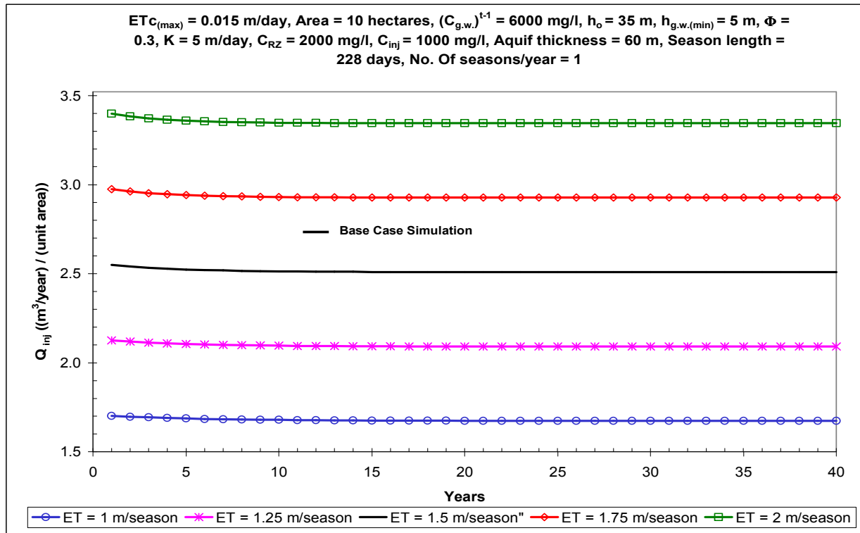
Figure 4. Amount of treated wastewater injected into the native groundwater for ranges of different actual crop evapotranspiration, ET c , input values vs. simulation period.
