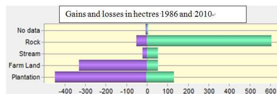
Figure 6. Gains and Losses in Hectares 1986-2010.
