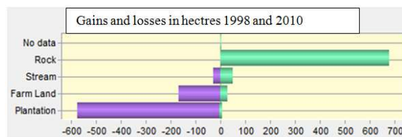
Figure 5. Gains and Losses in Hectares 1998-2010.
