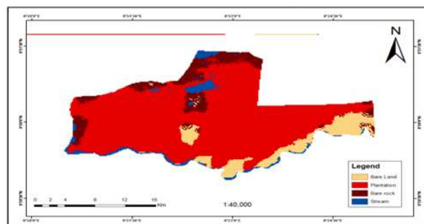
Fig 7. image showing landcover projection for 2037.
