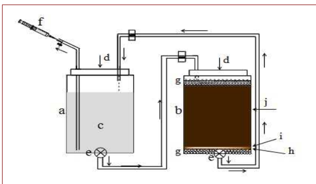
Figure 1. Experimental column set-up. a) Solution reservoir, b) sediment reservoir, c) media (effluent), d) \text{N}_2 , e) peristaltic pump, f) sampling syringe, g) glass beads, h) plastic grid, i) layer of sand, j) sediments.
