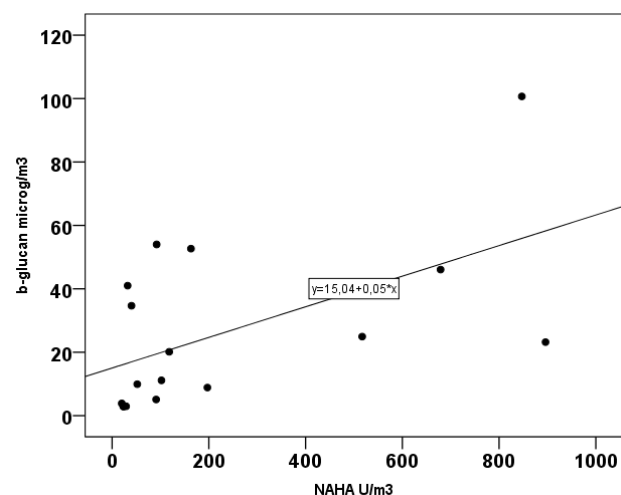
Figure 3. Relation between airborne NAHA ( \text{U/m}^3 ) and non-soluble \beta -glucan ( \text{microg/m}^3 ) extracted with 0.3 M NaOH ( p = 0.006 , Spearman's test).
