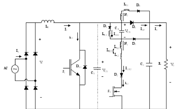
Figure 3. Circuit scheme for PFC converter implementing snubber circuit
