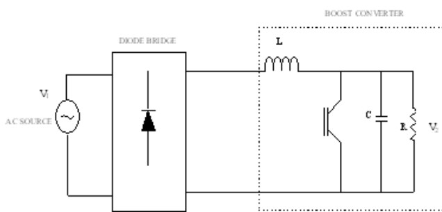
Figure 2. Passive topology of PFC
