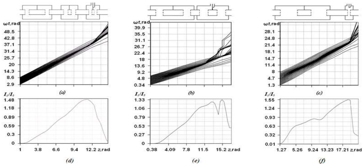
Fig. 2. Space-time diagram of electron motion and amplitude of a first harmonic of convection current: (a), (d) – three-cavity generating-amplifying klystron; (b), (e) – tristrion's; (c), (f) – two-cavity generating-amplifying klystron
