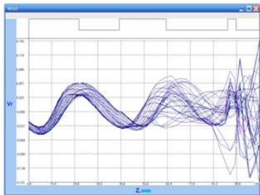
Fig 4. Relationships of longitudinal V_z (a) and radial V_r (b) normalized velocities from longitudinal coordinate z
