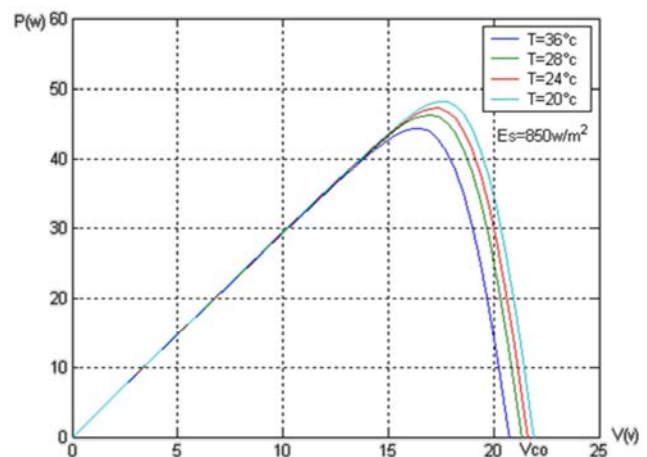
Figure 10. Influence of temperature on the characteristic P (V).
