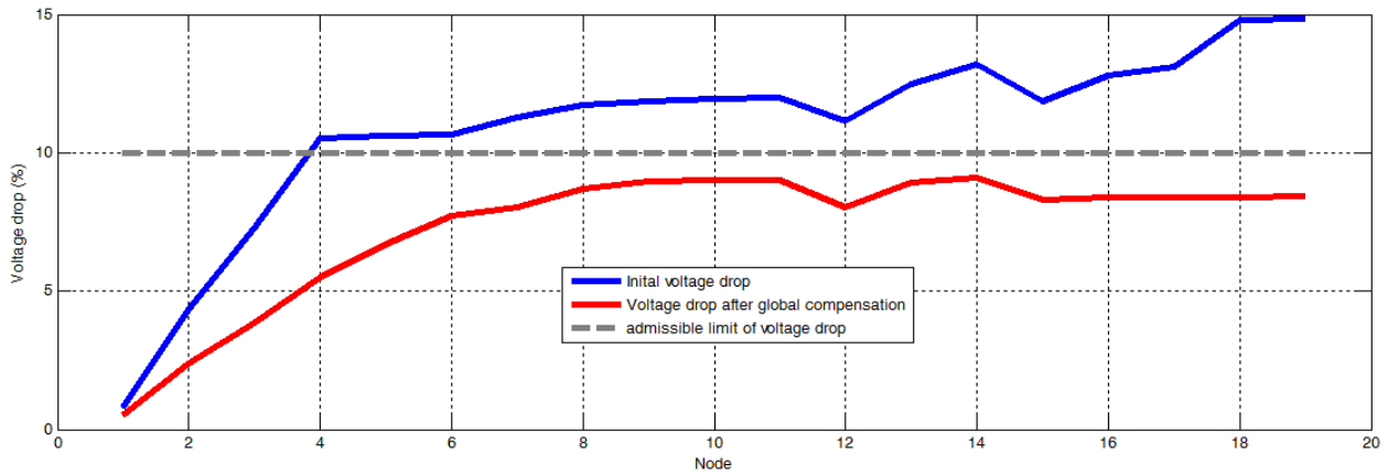
Figure 19. Voltage drops of departure N°2 after global compensation.
