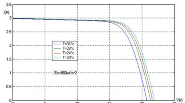
Figure 9. Influence of temperature on the characteristic I (V).
