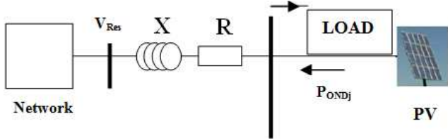
Figure 11. Model of a short line.
